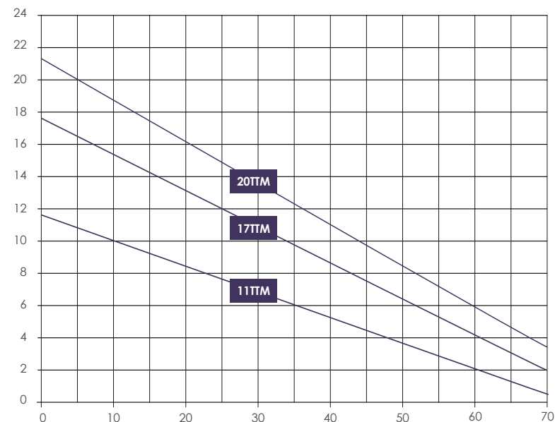
Temperature / Loading diagram TTM
