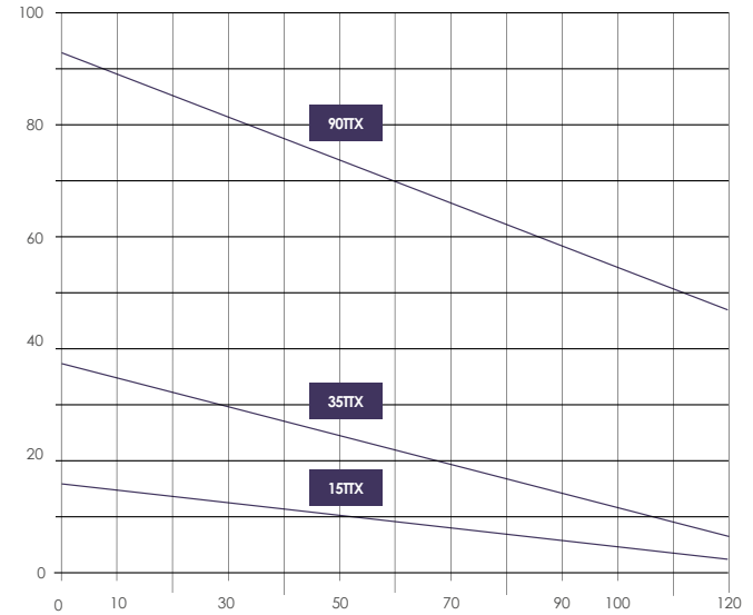
Temperature / Loading diagram TTM
